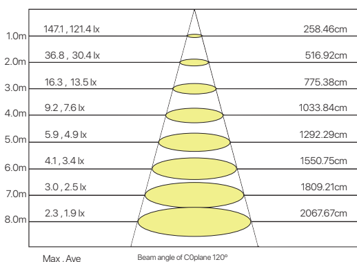
Lux Distance Curve
